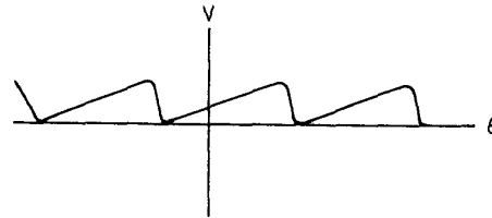
FIG. 3. A potential which violated V(\theta) .
