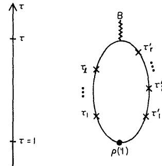
FIG. 4. Graphical notations. Solid lines represent propagating state vectors. Crosses represent the action of V . The black dot represents the initial density matrix and the wavy line represents the measurement of baryon number.
