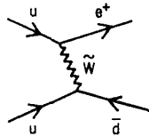
FIG. 1. Baryon-number-violating process occurring in the SU_5 's unified theory.
