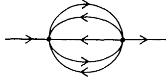
FIG. 2. Graph contributing to baryon dissipation.
