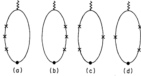
FIG. 6. The third-order contributions to \langle B(\tau) \rangle .
