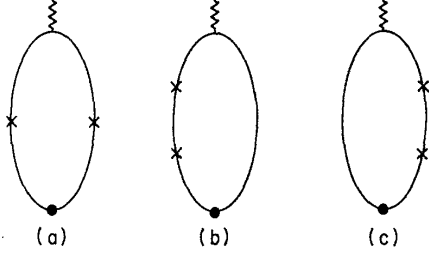
FIG. 5. The second-order contributions to \langle B(\tau) \rangle .
